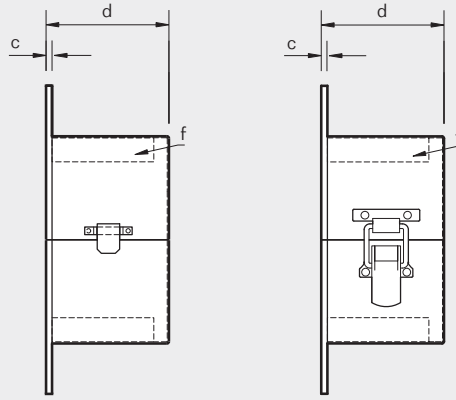
Tab fixing (≤ 40 mm/1.575")
